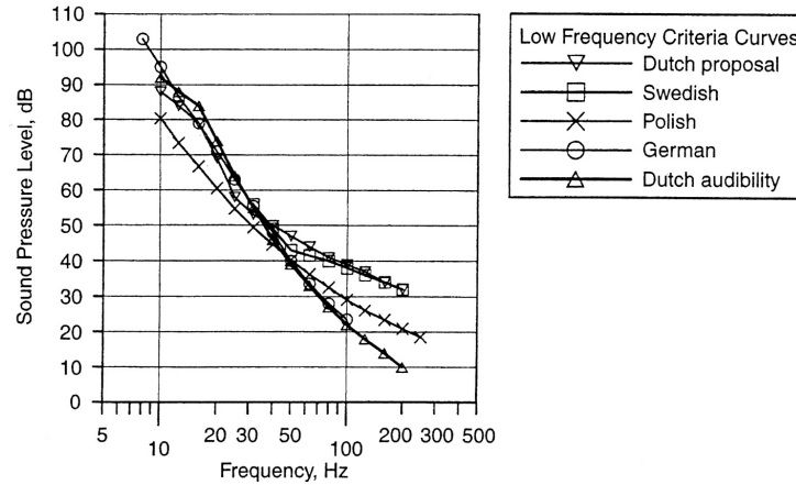
Figure 3 European Low Frequency Noise Criteria (after Poulsen 2003)
