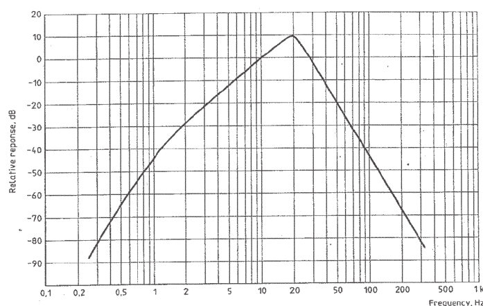
Figure 2 The G weighting (after ISO 7196:1995)
