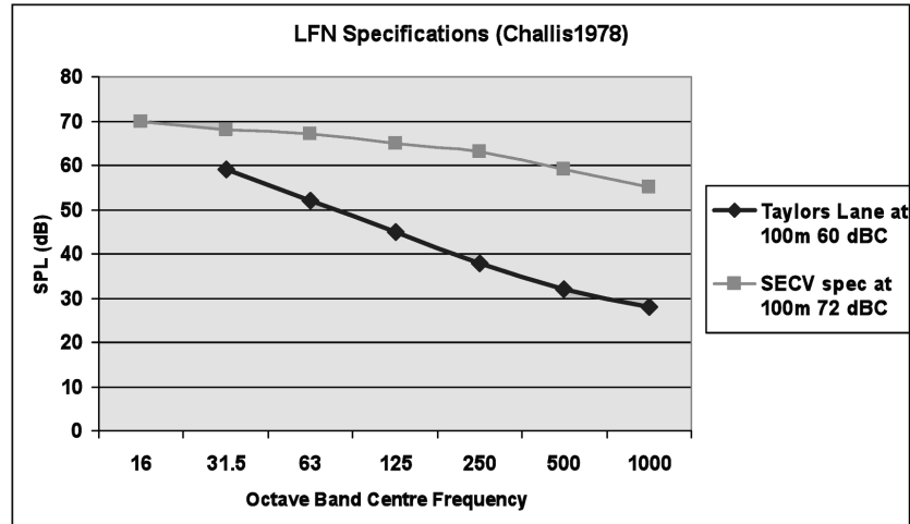
Figure 5. LFN specifications by utilities quoted by Challis
