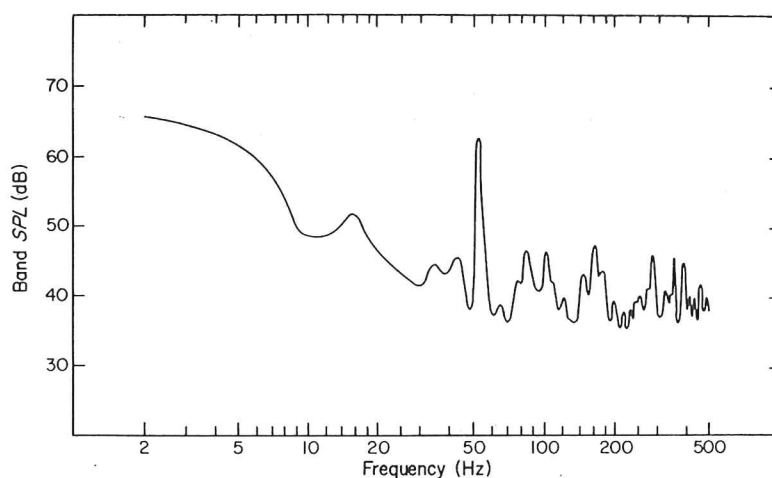
Figure 1. Noise spectrum (2 Hz constant bandwidth) measured in a bedroom and which caused annoyance.
