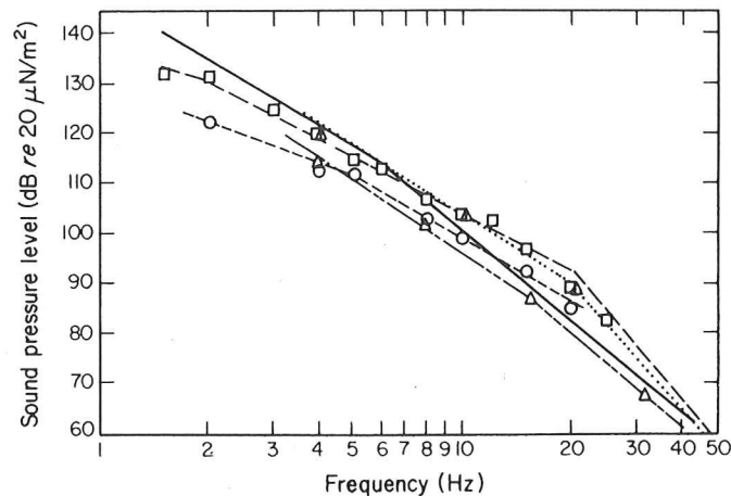
Figure 3. Hearing threshold levels for maximum audible pressure (MAP), minimum audible field (MAF) and for bands of noise (after Nixon and Johnson [51]). —, Bekesy, MAP; \square , Yeowart, MAP; \circ , Yeowart, MAF; \triangle , Yeowart tone threshold; \nabla , Yeowart, noise threshold.
